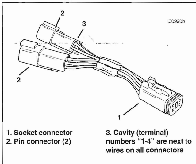
Illustration. Two-Into-One Harness Adapter
